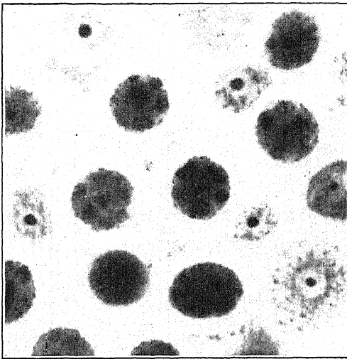
Ameba limax . Aggregations of idiochromidia to form sixteen secondary nuclei, which then unite to form eight.
